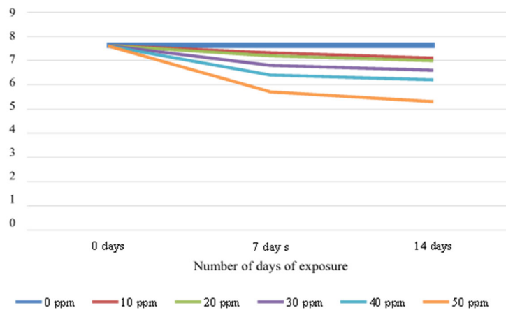
Fig. 4. Effect of PH on the reduction of chlorophyll of A. microphylla during the study
