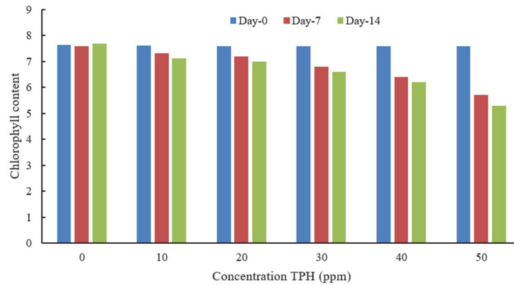
Fig. 3. Effect of petroleum hydrocarbons on chlorophyll of A. microphylla
